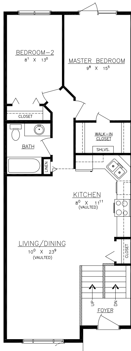
FLOOR PLAN
